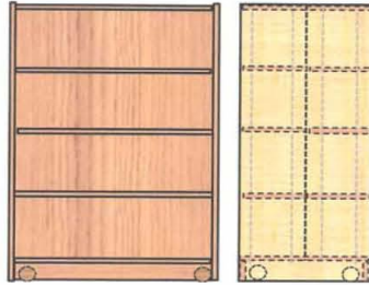
NO. 3L108 DOUBLE FACE MOBILE 36"W X 60"H X 24"D
