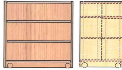
NO. 3L109- DOUBLE FACE MOBILE 36"W X 48"H X 24"D
