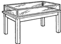
No. 3L365 Display Table Oak Aprons & Legs w/1/4" plate glass sides and hinged top in a aluminum frame 60" w x 30" d x 36" h overall
