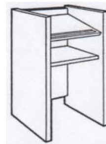
No. 3L344 LECTERN 26"w x 21"d x 44"h 1-1/8" thick ends/adj. glides
