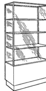
No. 3L369 Display Case 3/4" Oak plywood base w/1/4" plate glass sides , shelves & top in a aluminum frame 42" w x 16" d x 84" h
